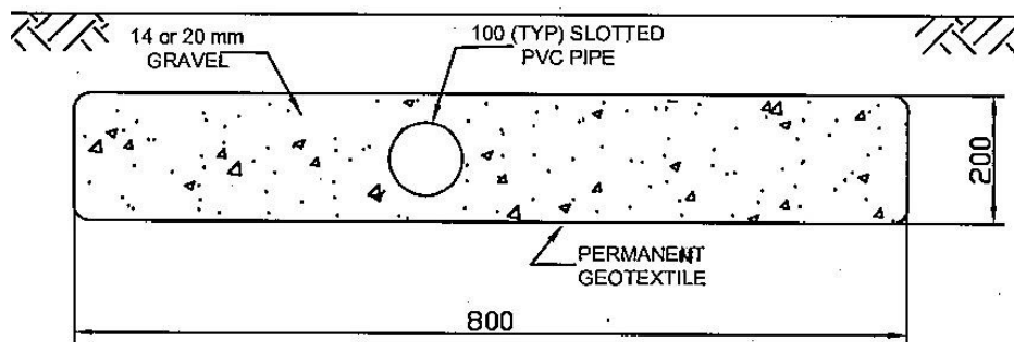
Figure 5 – Groundwater Recharge Trench, Section
