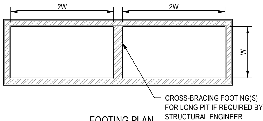
FOOTING PLAN
