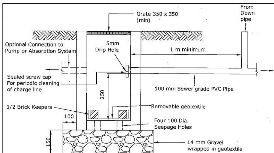
Figure 3 – Charged Pipe Cleanout Pit
