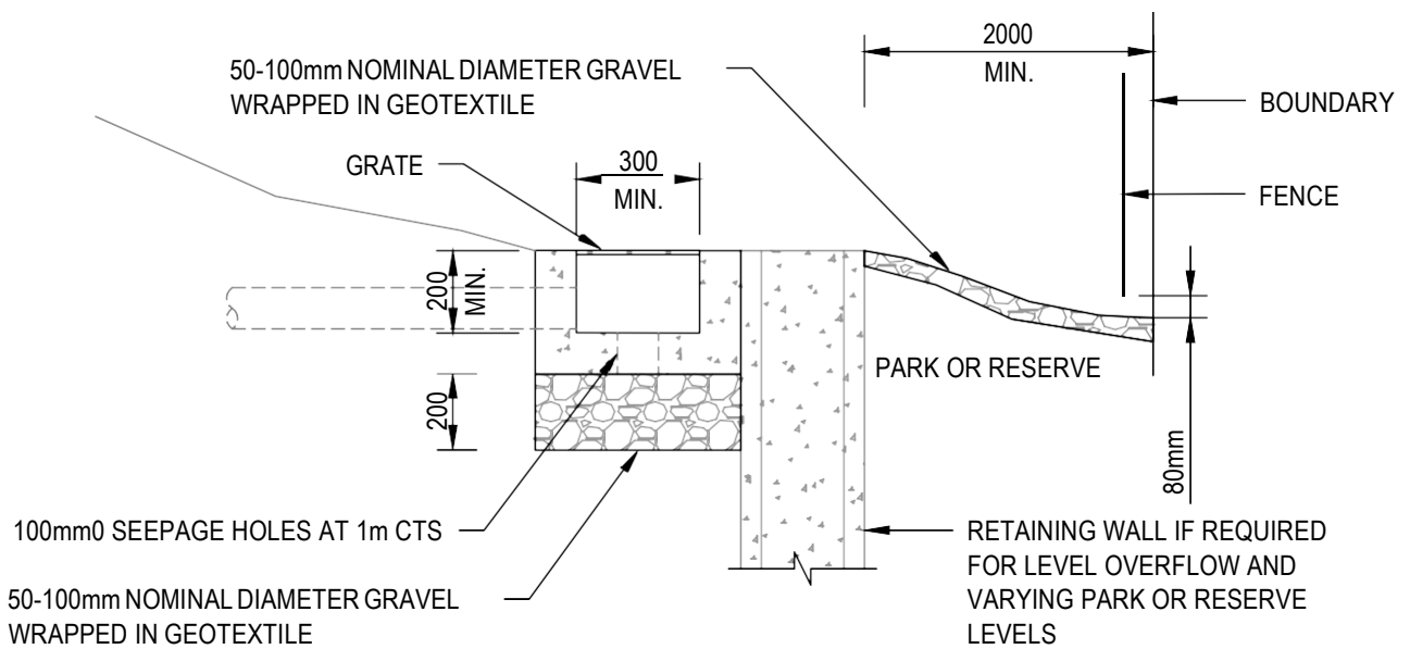
ELEVATION VIEW
